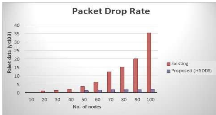
Figure 5: Comparative bar graph of packet drop rate (packet loss)
