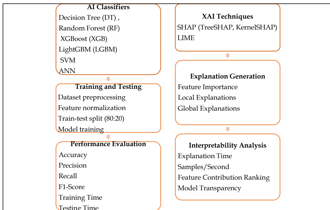
Figure 1: Methodology used for AI and XAI-Based Intrusion Detection
