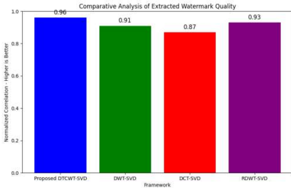
Figure 12. Cross Comparison of Extracted Watermark Quality
