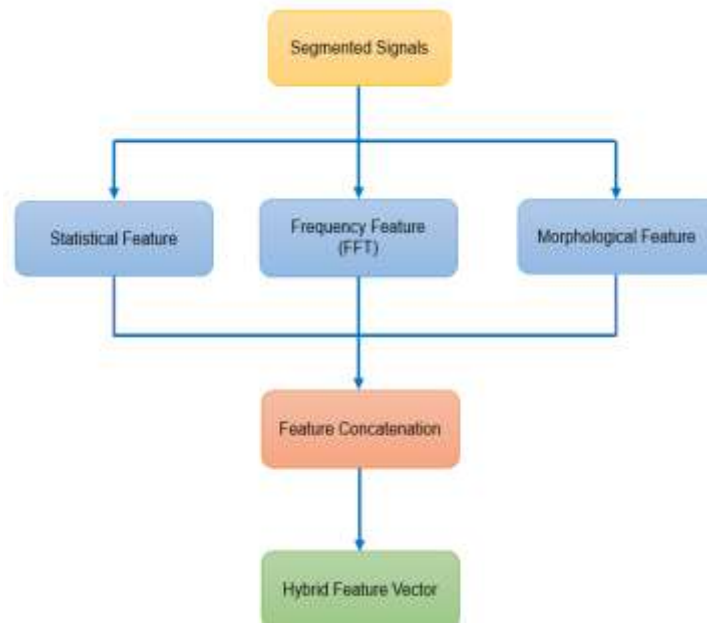
Figure 2: Hybrid Feature Extraction
