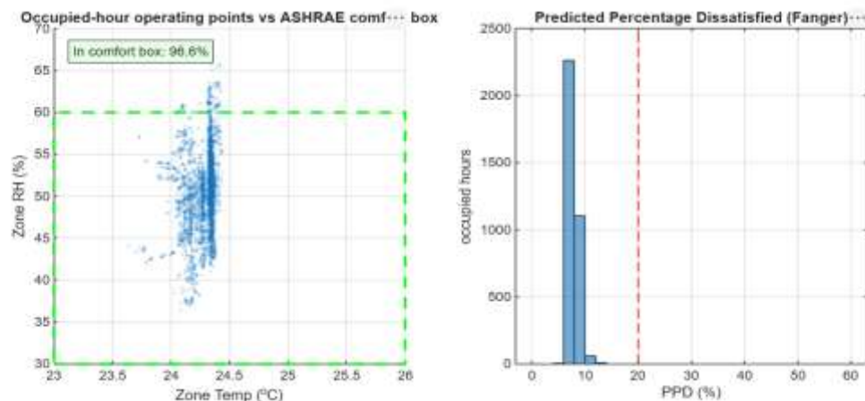
Figure 8. Locked controller, occupied hours. Left: operating points against the ASHRAE comfort box. Right: PPD distribution with the PPD = 20 threshold marked.
