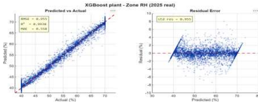
Figure 3. Zone relative humidity surrogate on real 2025 transitions.
