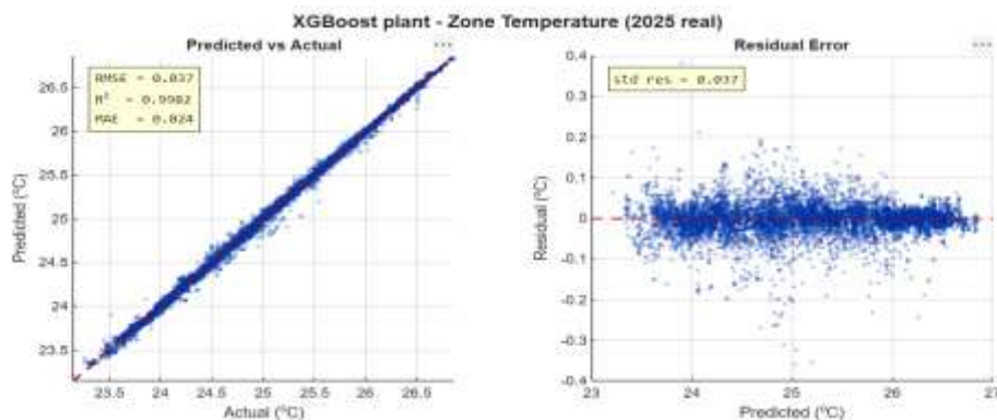
Figure 2. Zone temperature surrogate on real 2025 transitions: predicted versus actual (left), residuals (right).
