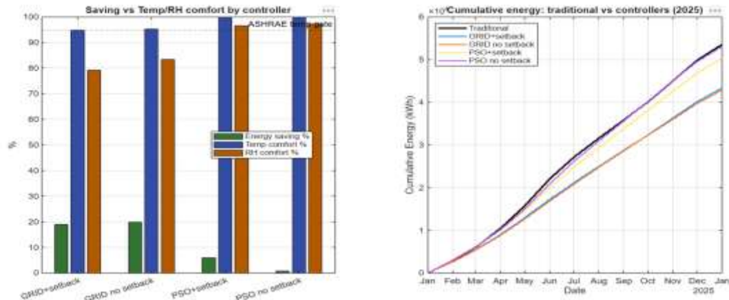
Figure 5. Controller comparison, 2025. Left: annual saving and occupied-hour temperature and humidity compliance for all four, with the 95% temperature gate marked. Right: cumulative annual energy, baseline and all four controllers.
