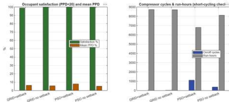
Figure 6. IEQ and hardware comparison. Left: occupant satisfaction and mean PPD. Right: compressor cycles and run-hours — the short-cycling check.
