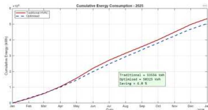
Figure 7. Cumulative 2025 energy, baseline against the locked controller.
